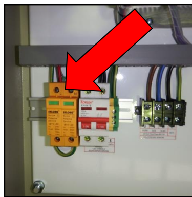
Installed surge arrester in SD75 Cartridge indicator; Green is good, Red is blown
