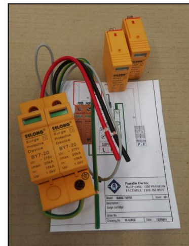
Retrofit Kit; Surge Arrester with wiring loom, connect diagram, spare cartridges, Order # 313 000 206
