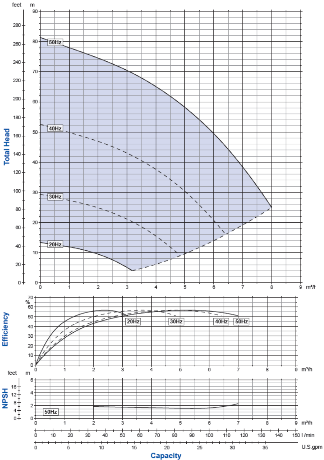
Performance Curve 20 to 50 Hz, FPS MHQP
